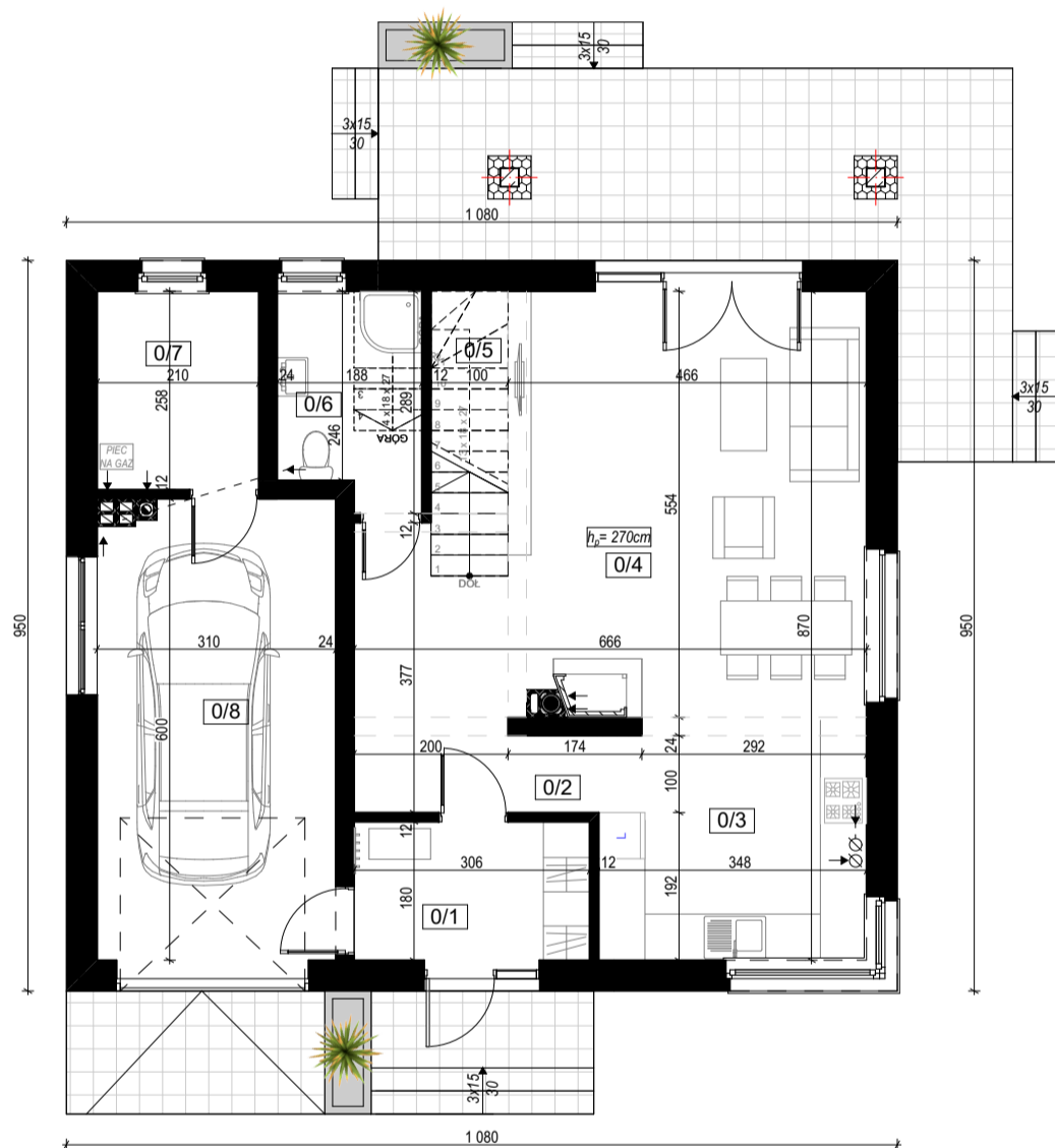
PARTER
